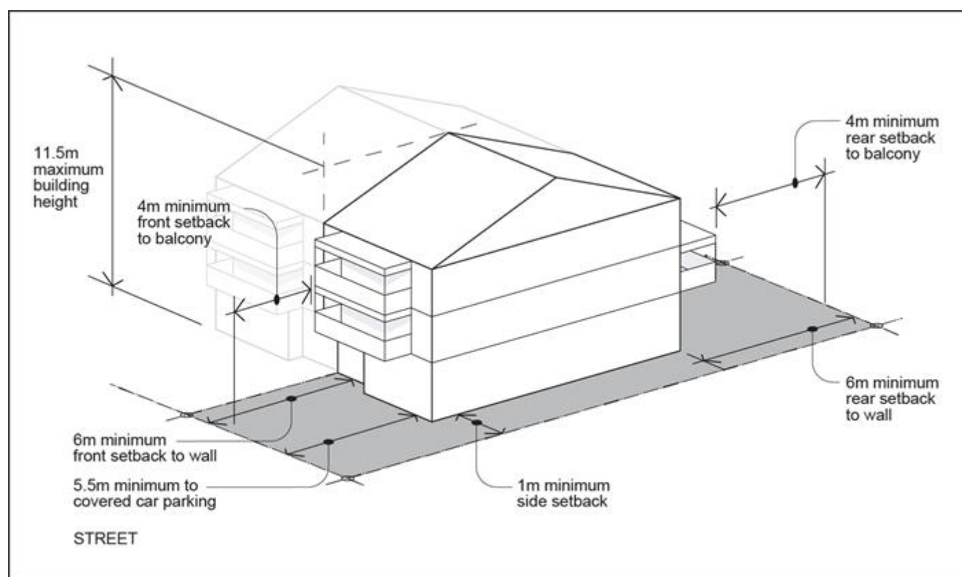
Figure k—Building envelope for lots under 180m 2 with a lot depth greater than 25m
