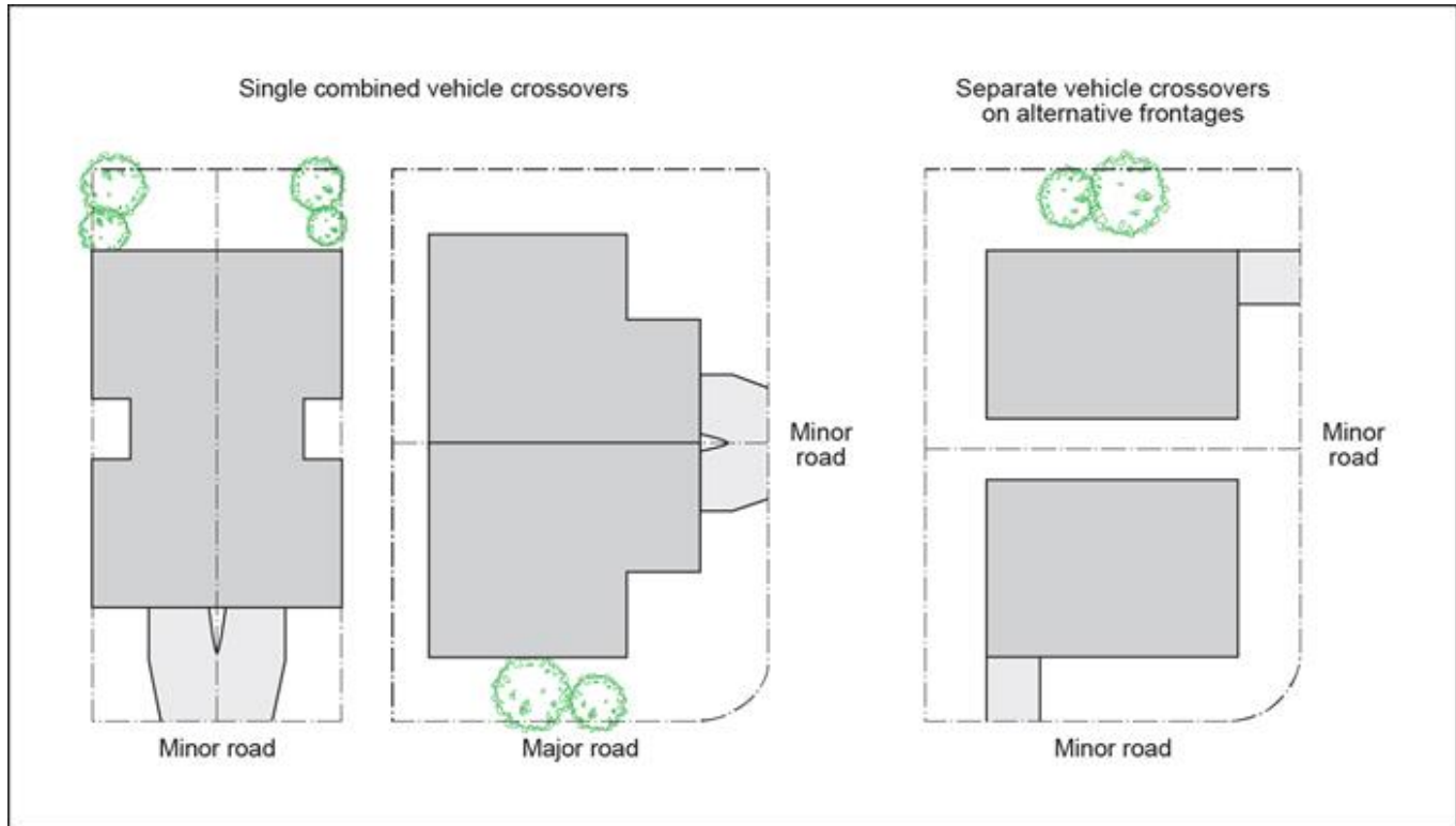
Figure o—Example crossover arrangements
