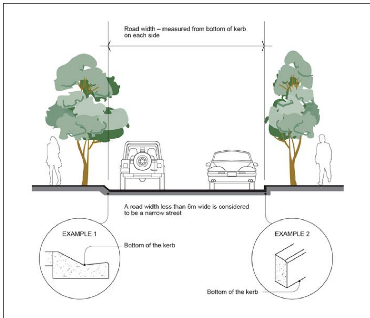
Figure g—Measurement of a narrow street
