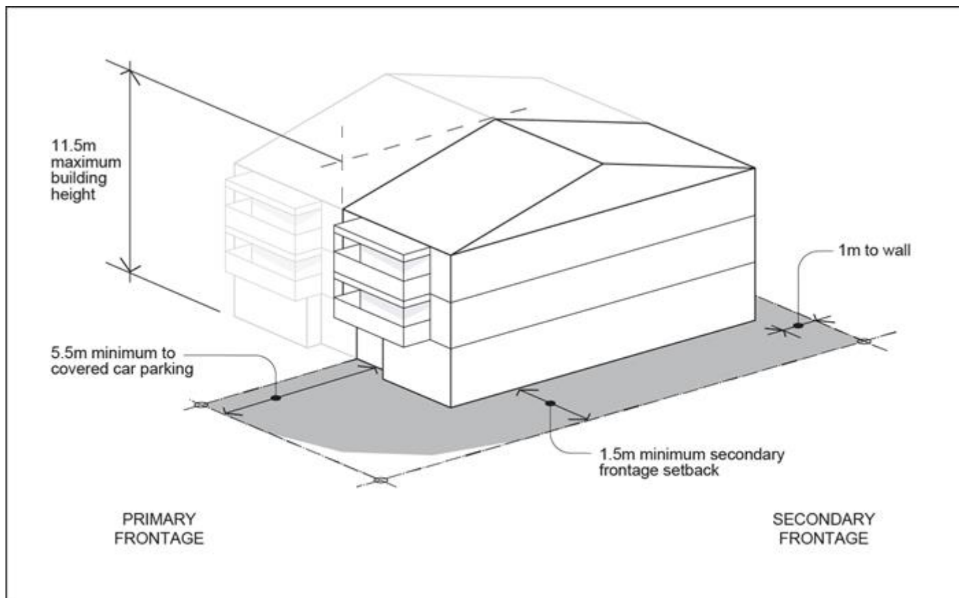
Figure I—Building envelope for lots under 180m² (corner lot)
