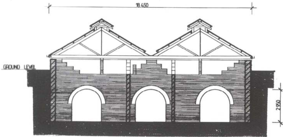
RESERVOIR No1. - Section A-A
